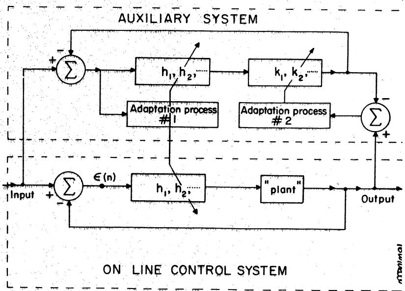
Fig. 10 Data-Repeating With Auxiliary System
