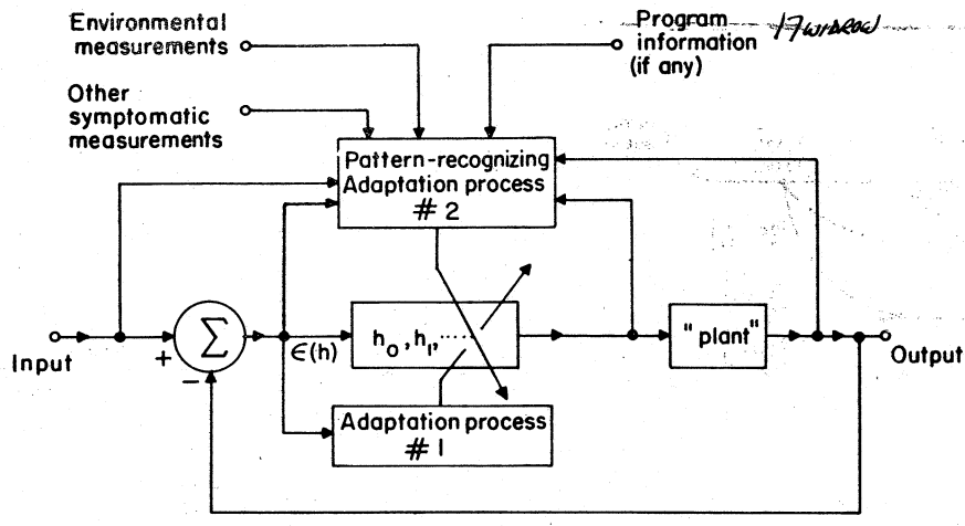
Fig. 11 Pattern-Recognizing Adaptive Feedback System
