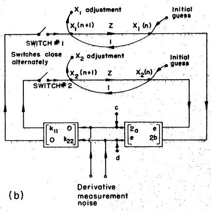
Fig. 7 Feedback Models of Two-Dimensional Surface-Searching
