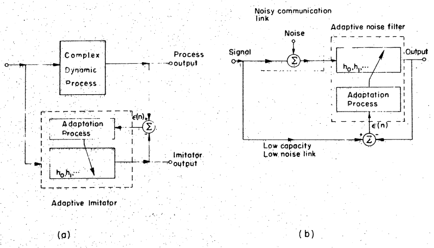
Fig. 8 Adaptive Noise Filter and Adaptive Learning Process
