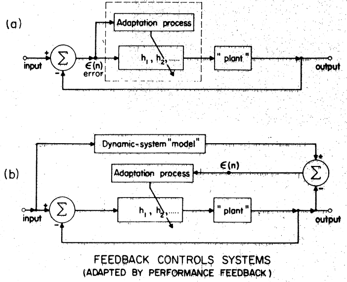
Fig. 9 Adaptive Feedback Systems; Model-Reference Adaptation
