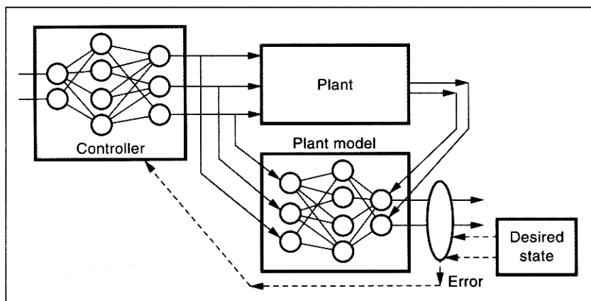
Figure 10. Adaptive plant emulation. Source: Courtesy of Jim Keeler
